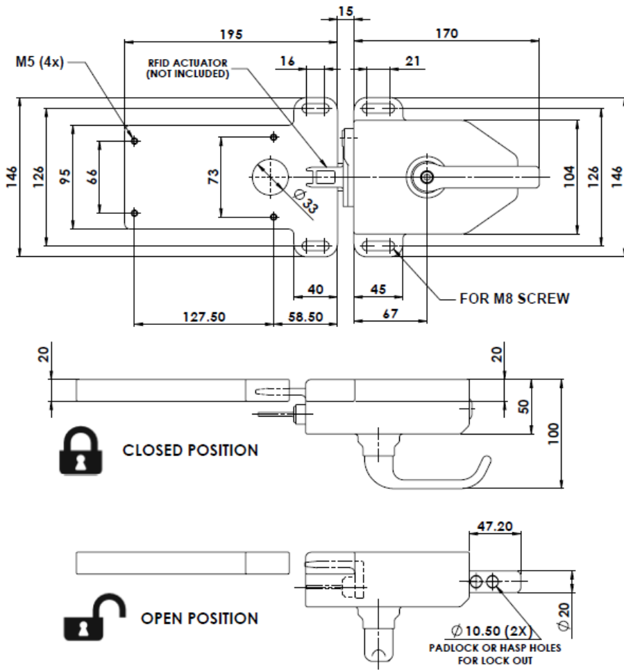
Product Dimensions – Type: UGB 2 Rotary Handle SS (2 x APP)
